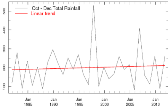
Figure 6: Tana River OND Season 1981-2011
