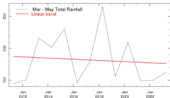
Figure 17: Tana River Mean RF 2011-2041 March- May
