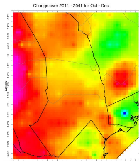
Figure 20: Tana River Mean RF 2011-2041 Oct-Dec
