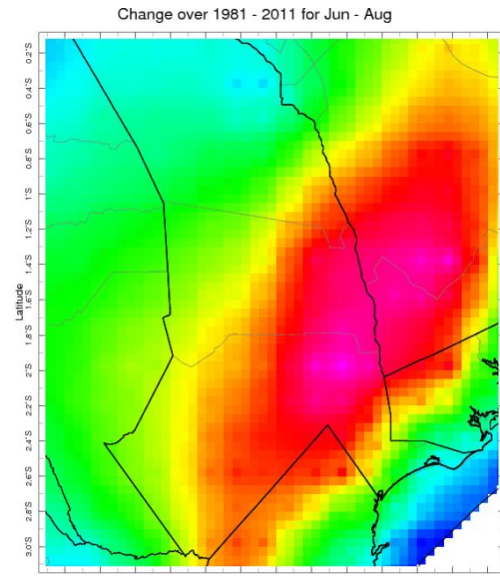
Figure 14: Tana River mean Temp 1981-2011 (Jun-Aug)
